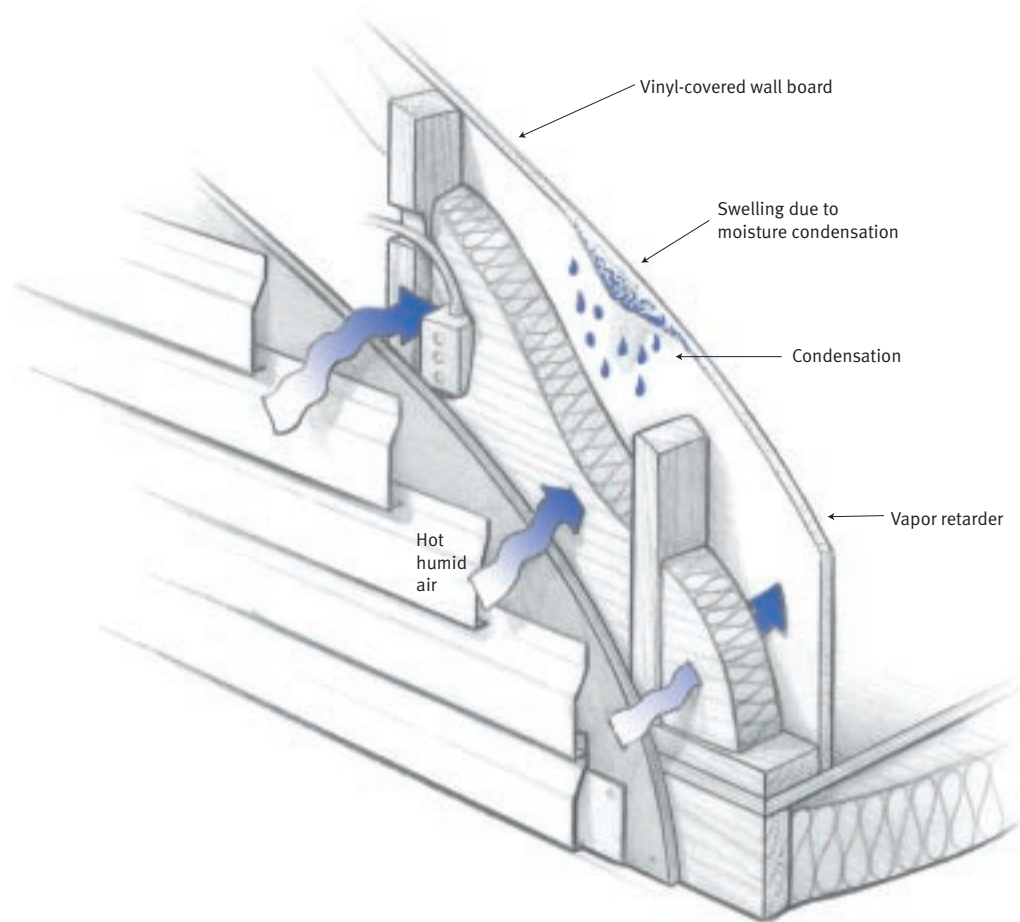
Figure 3.5 Vapor Retarder on the Wrong Side
