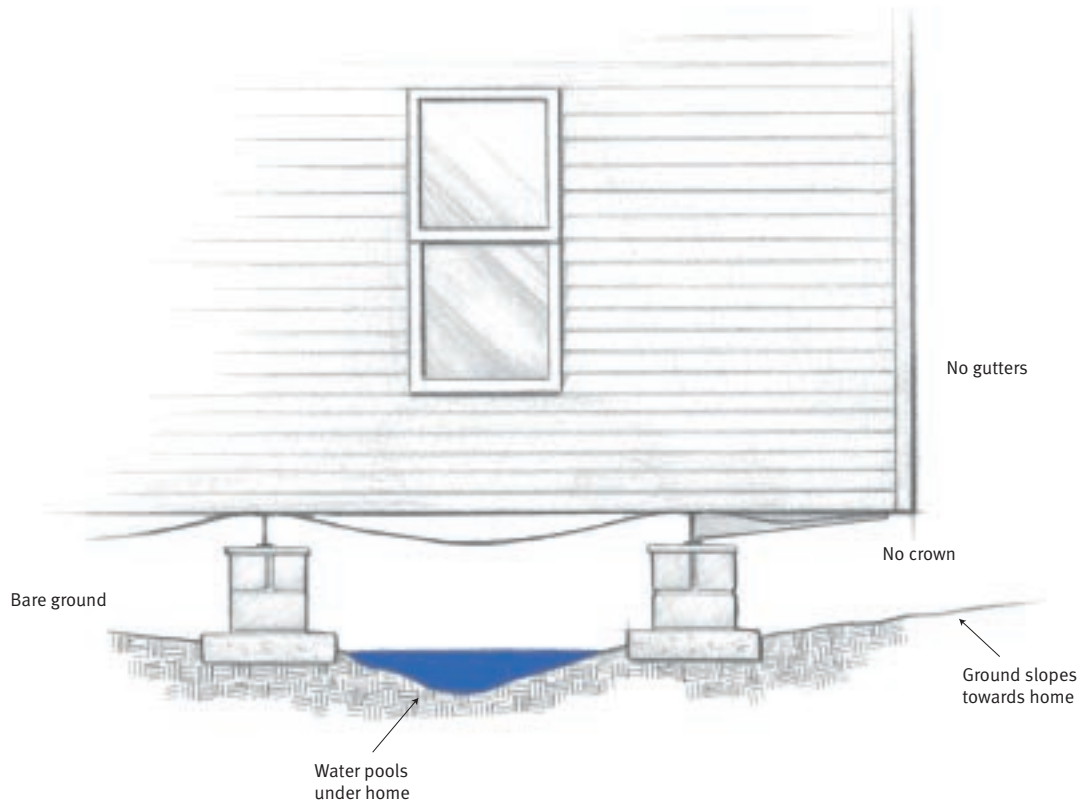
Figure 2.5 Site Grading Practices to Avoid
